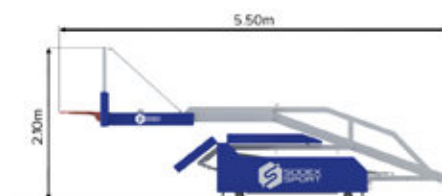
Storage position
